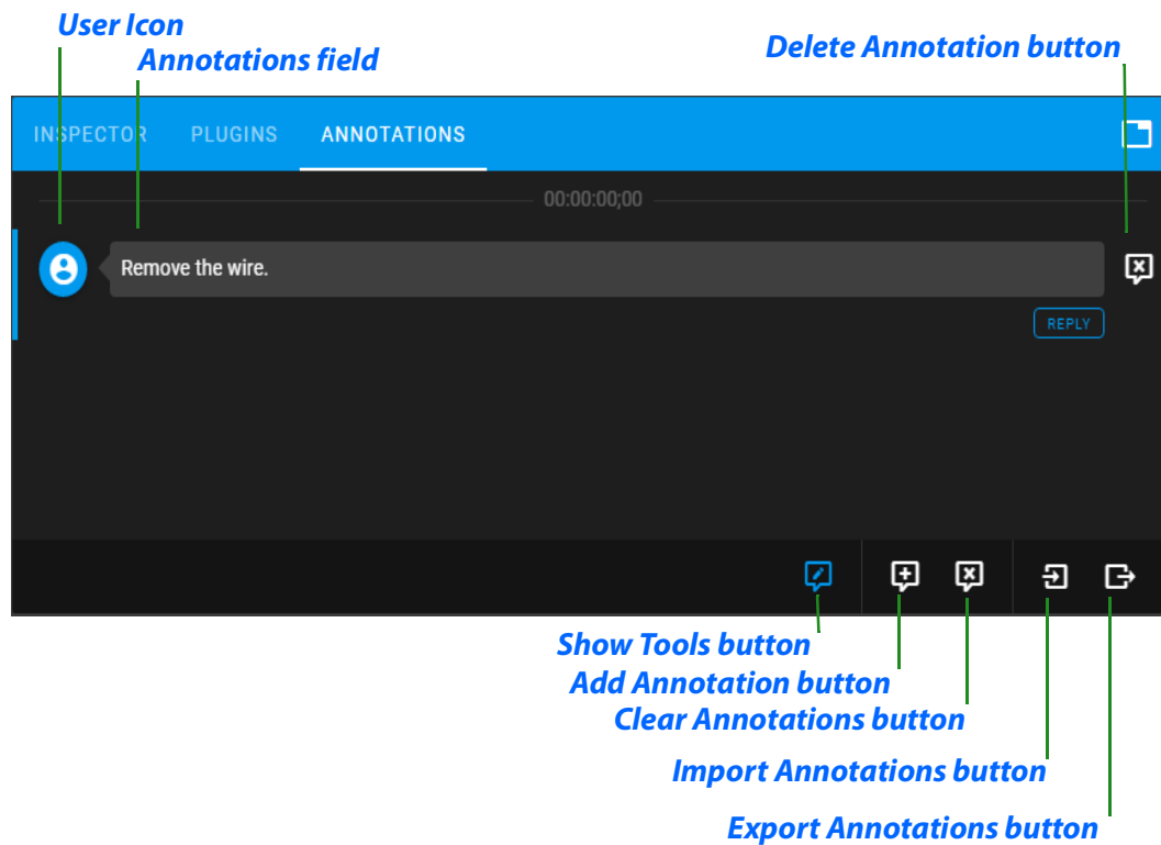
Figure 6. Annotations Tab
