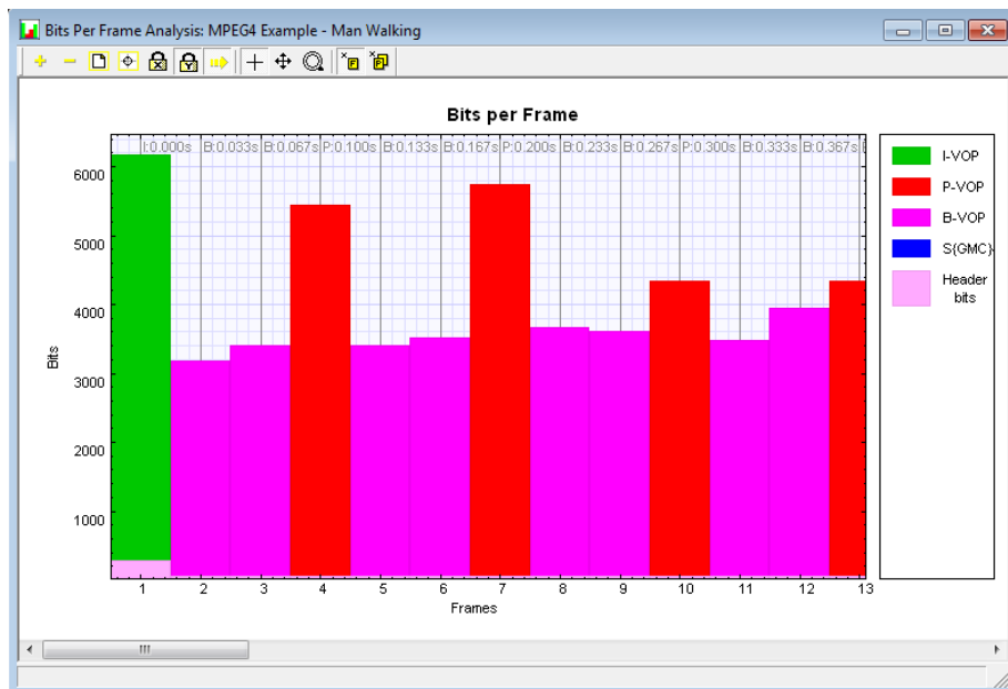
Figure 32: Bits per Frame Analysis graph – MPEG-4 example
