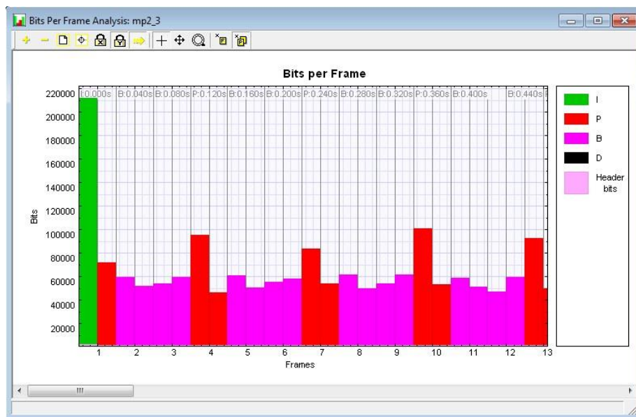
Figure 35: Bits per Frame Analysis graph – MPEG-2 example of Picture units display
