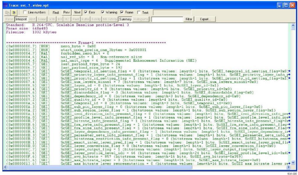
Figure 16: H.264/SVC example, at start of byte stream (full MTS4EA Trace view window)
