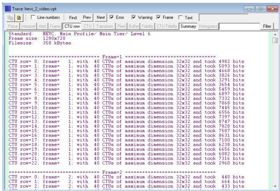
Figure 21: H.265 example
