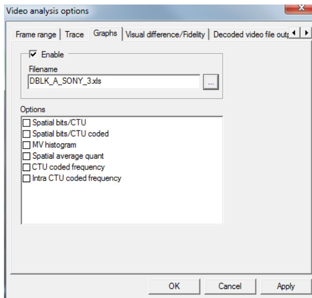
Figure 27: H.265 graph
