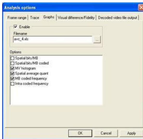
Figure 26: H.264 graph
