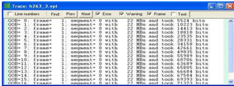
Figure 20: H.263 example
