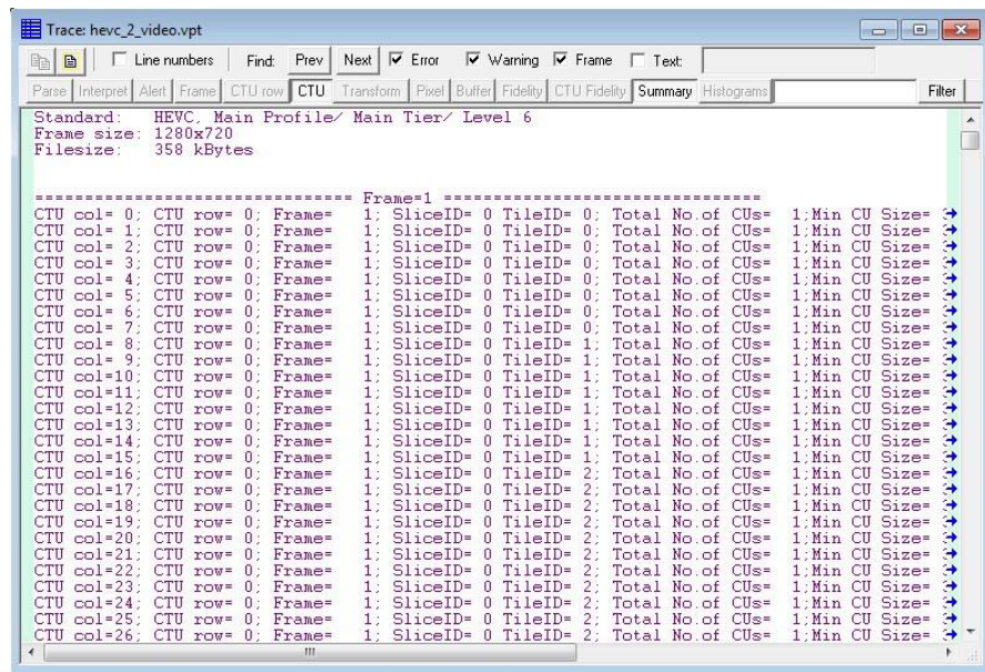
Figure 24: H.265 example
